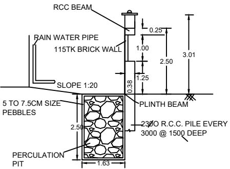
RAINWATER HARVESTING
