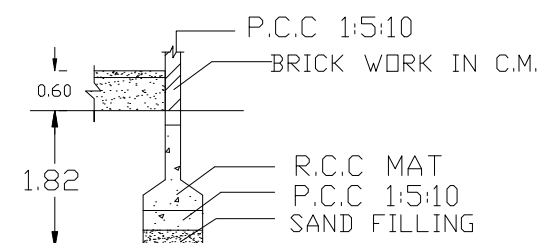
FOUNDATION DETAILS
