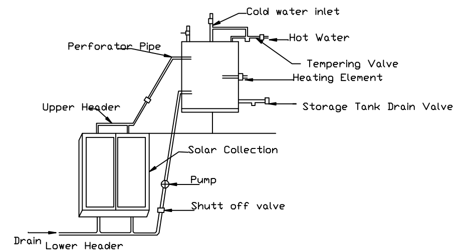
Details Of Solar Water Heater (NTS)
