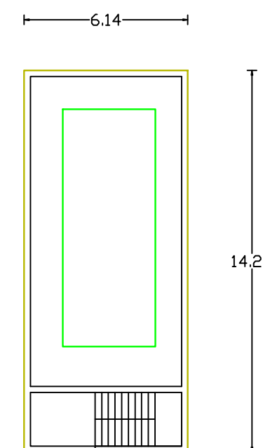
FLOOR-TERRACE
