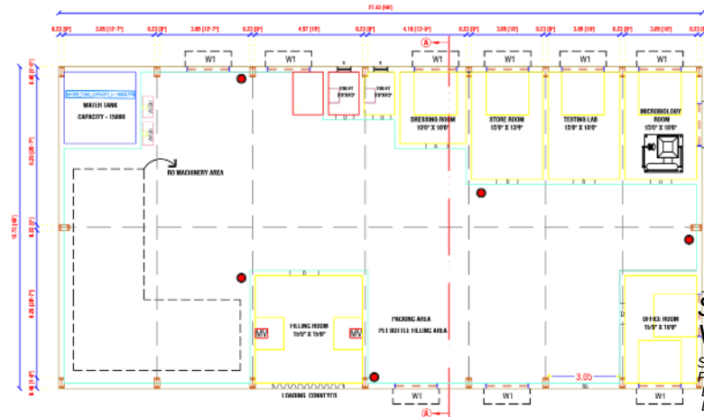
PROPOSED BUILDING GROUND FLOOR
