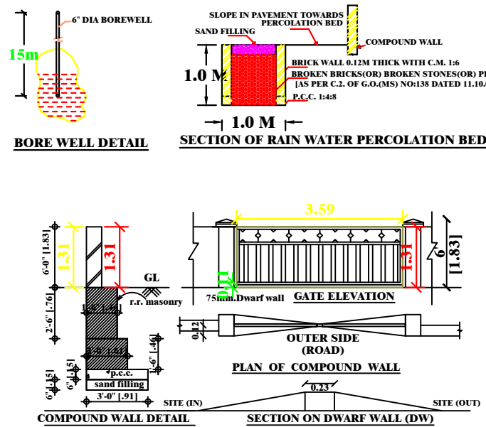
PLAN OF COMPOUND WALL
