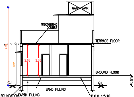
SECTION 'X-X'
