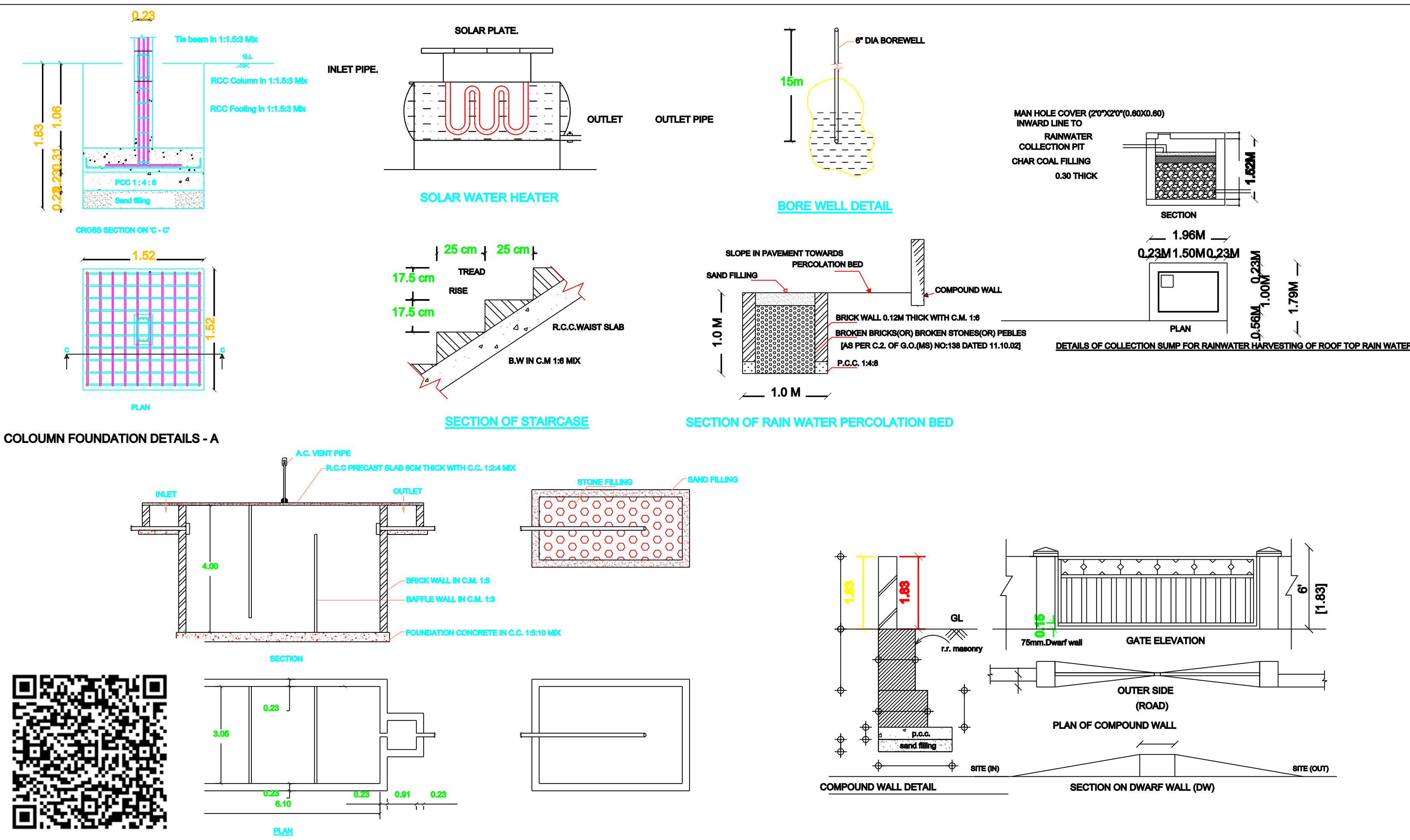
SECTION OF SEPTIC TANK & DISPERSION TRENCH
