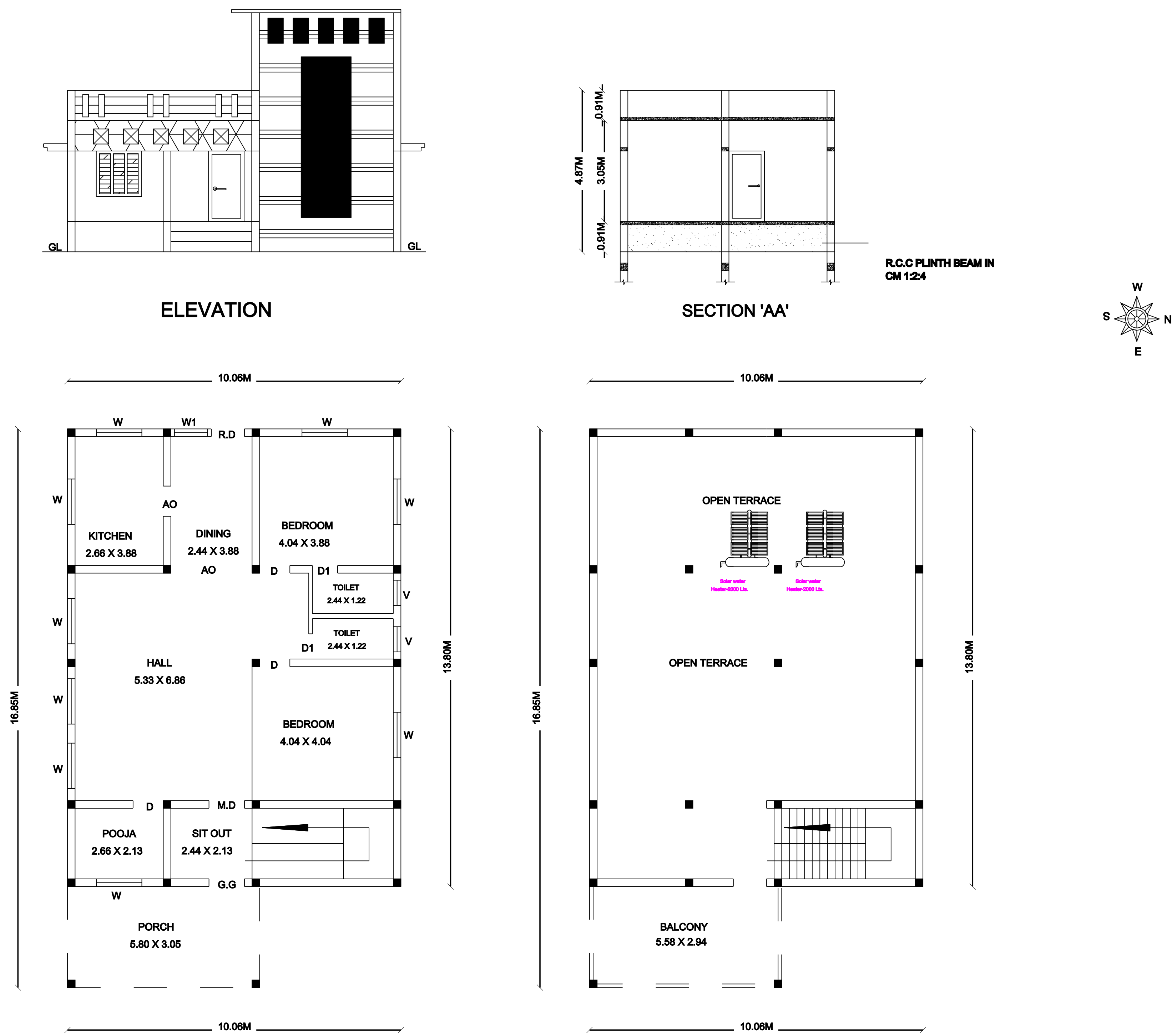
TYPICAL GROUND FLOOR PLAN
