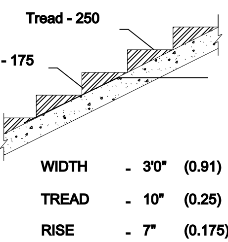
STAIR-CASE DETAILS (NOT TO SCALE)
