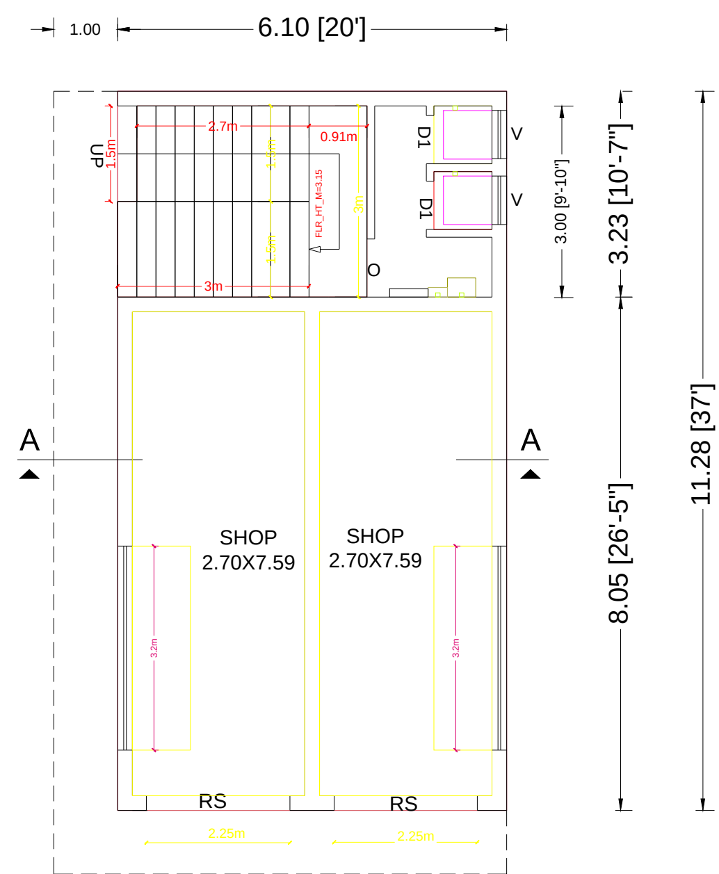
GROUND FLOOR PLAN FACING NORTH
