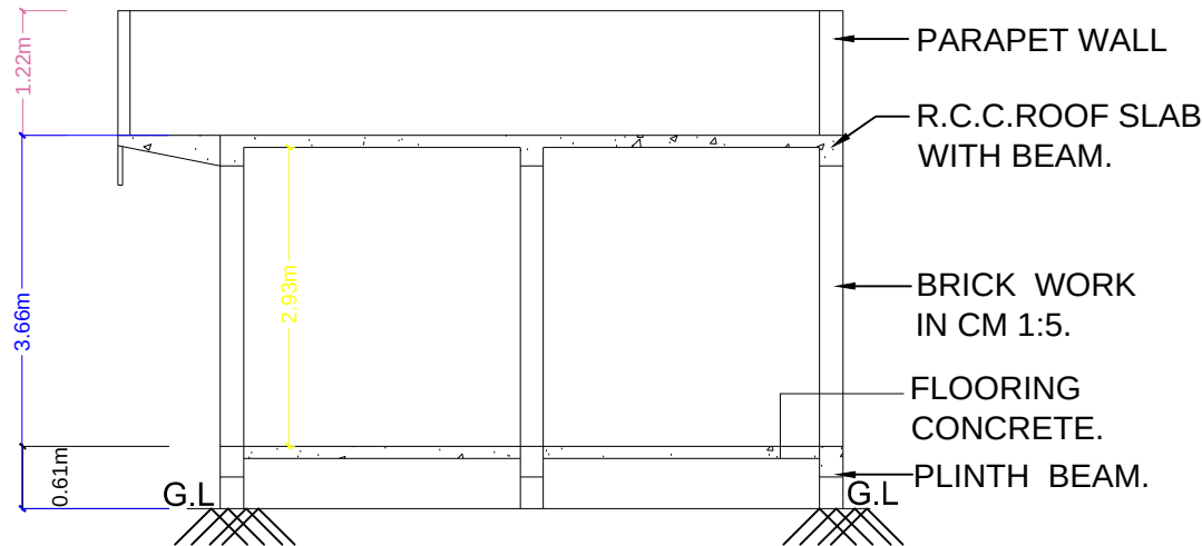
CROSS SECTION ON AA
