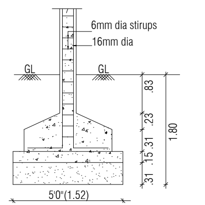
COLUMN FOUNDATION SCALE (1:50)
