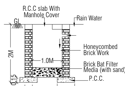
DETAILS OF RAIN WATER COLLECTION PIT SCALE:- 1"=4'0"
