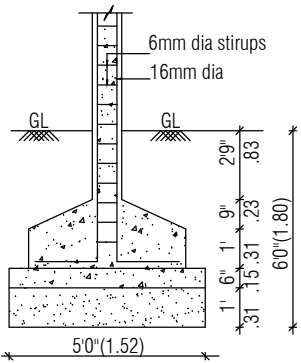
FOUNDATION DETAIL
