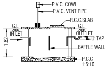
SEC. OF SEPTIC TANK"AA"
