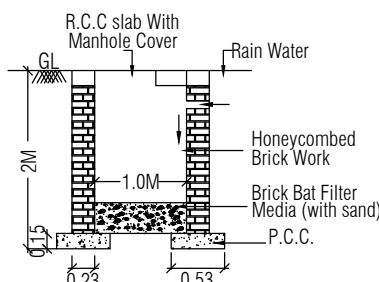
DETAILS OF RAIN WATER COLLECTION PIT
