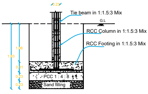
CROSS SECTION ON 'C - C'
