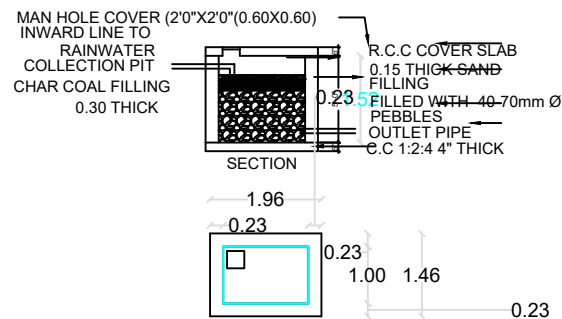
RWH_CAPACITY_L=5000LTRS
