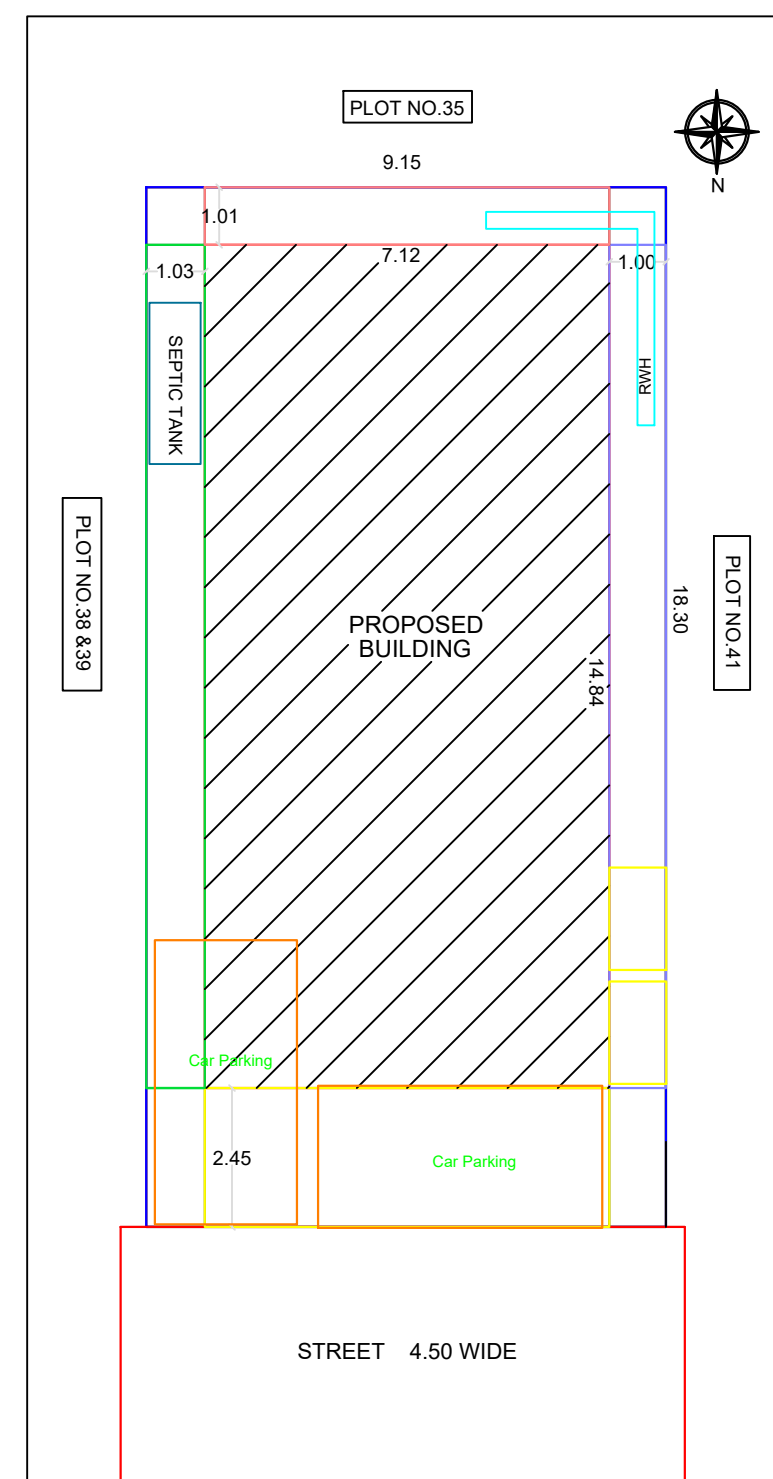
SITE PLAN
