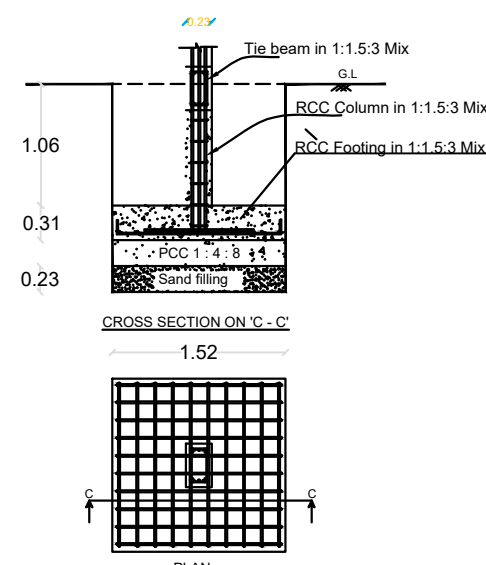
COLOUMN FOUNDATION
