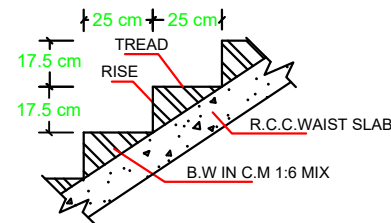
SECTION ON DWARF WALL (DW)
