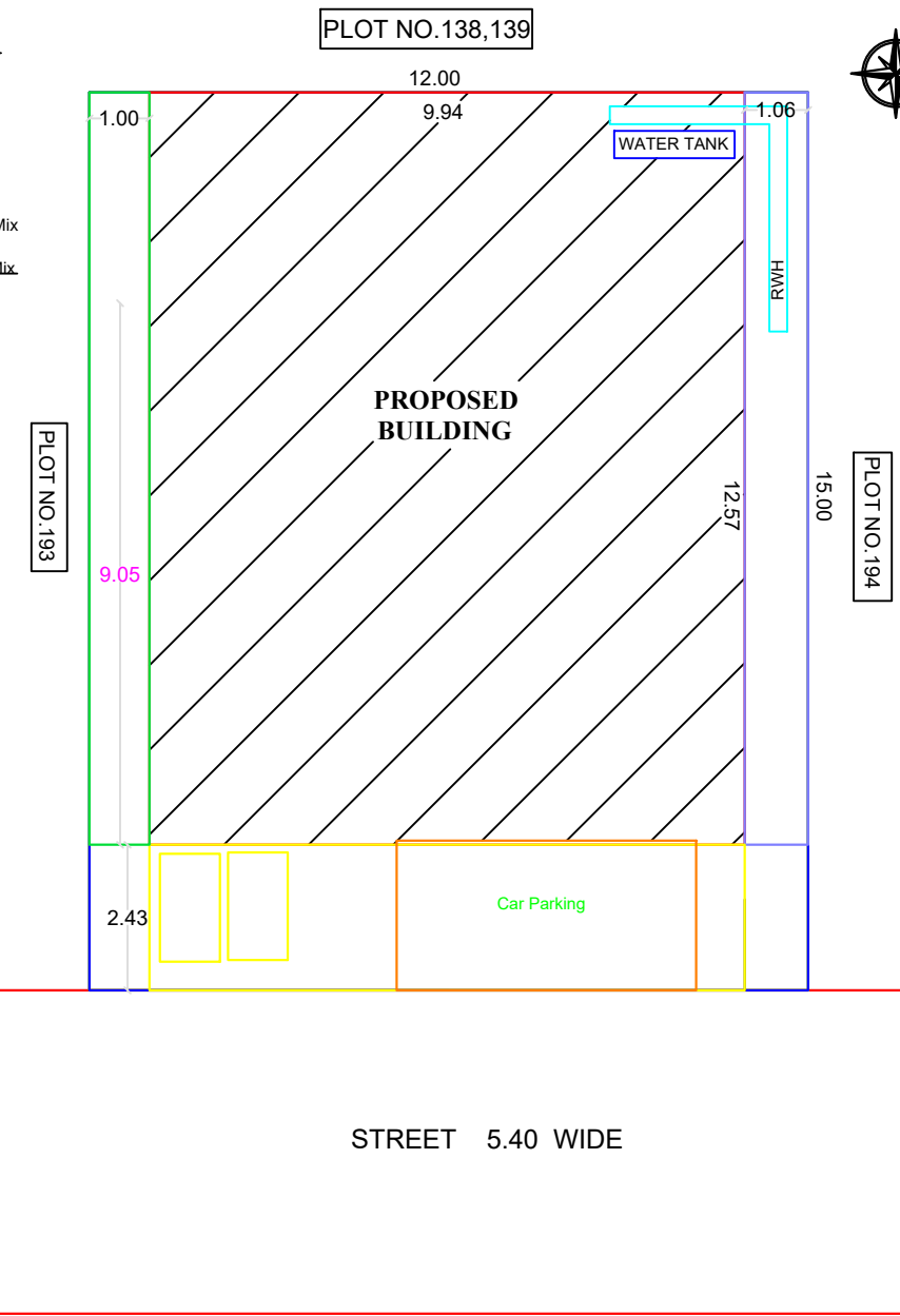
SITE PLAN
