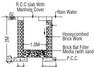
DETAILS OF RAIN WATER COLLECTION PIT SCALE:- 1"=4'0"
