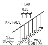
STAIRCASE DETAILS
