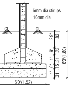
FOUNDATION DETAIL SCALE (1:50)
