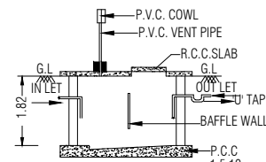
SEC. OF SEPTIC TANK"AA"
