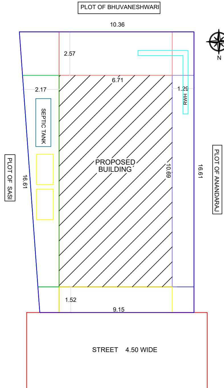
SITE PLAN
