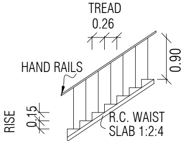
STAIRCASE DETAILS
