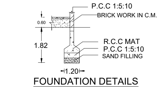
FOUNDATION DETAILS
