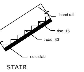
STAIR
