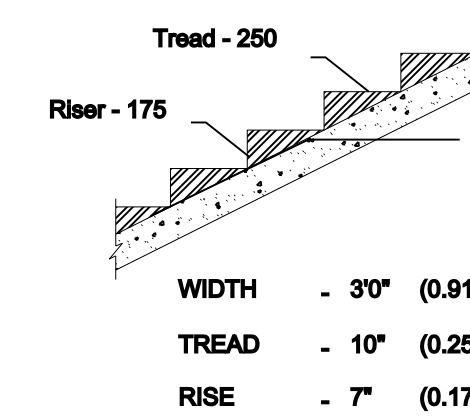
STAIR-CASE DETAILS ( NOT TO SCALE )
