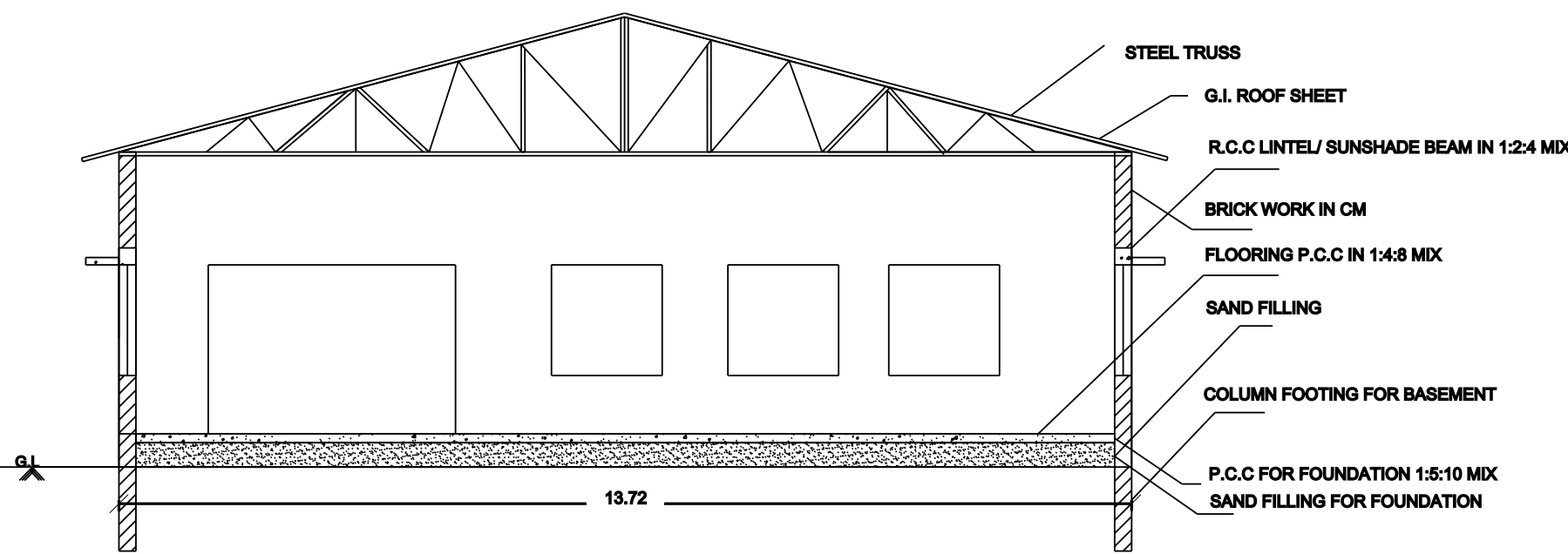
SECTION ON-AA
