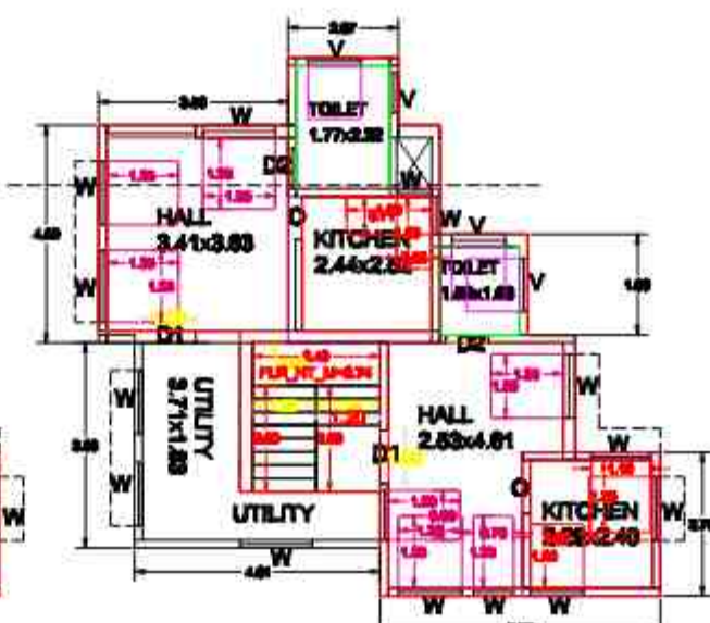
SECOND FLOOR(EXISTING)
