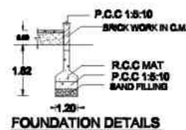
FOUNDATION DETAILS
