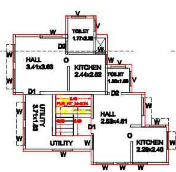
SECOND FLOOR(EXISTING)
