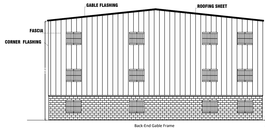
Back-End Gable Frame ELEVATION
