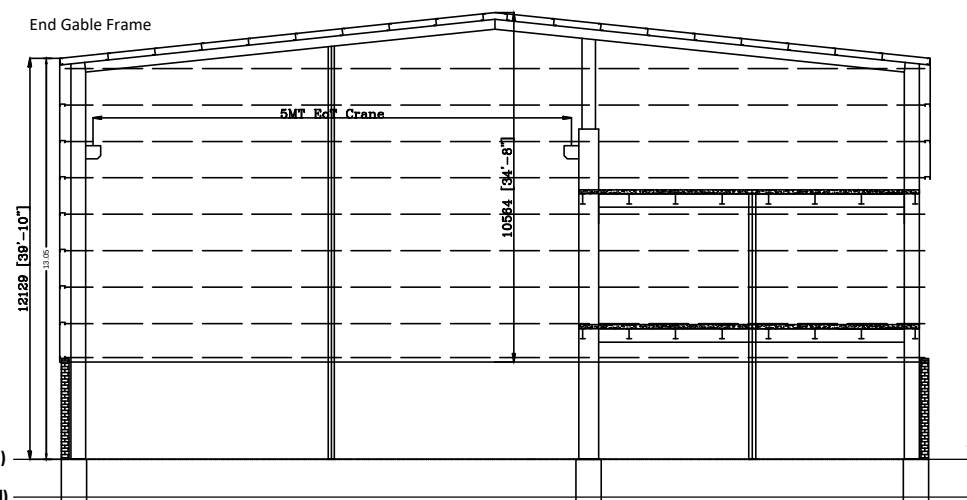
SECTION
