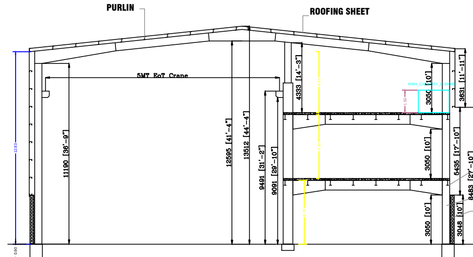
SECTION
