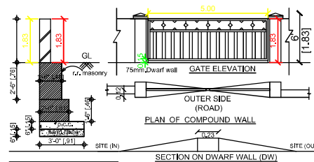
SECTION ON DWARF WALL (DW)
