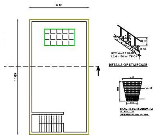
TERRACE FLOOR
