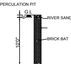
PERCOLATION PIT
