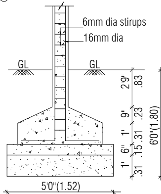
FOUNDATION DETAIL
