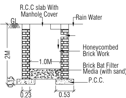
DETAILS OF RAIN WATER COLLECTION PIT SCALE: - 1" = 4'0"
