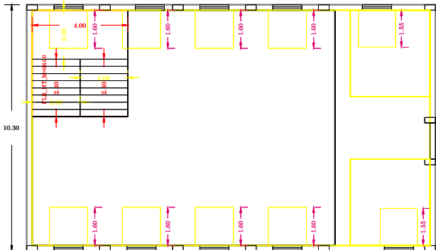
PROPOSED FIRST FLOOR PLAN BLOCK-1
