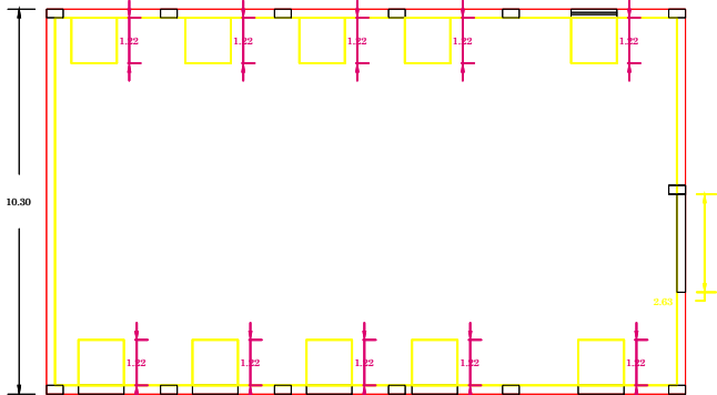
PROPOSED GROUND FLOOR PLAN BLOCK-2
