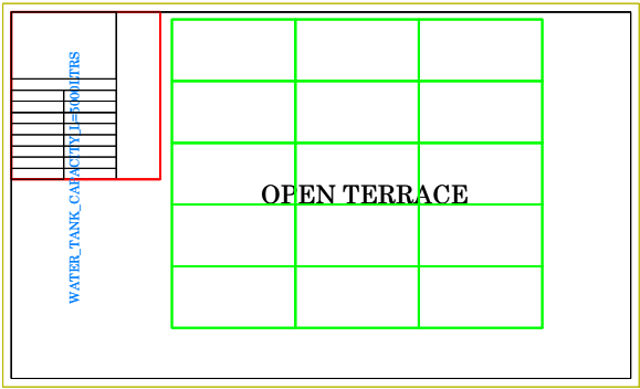
PROPOSED TERRACE FLOOR PLAN BLOCK-1
