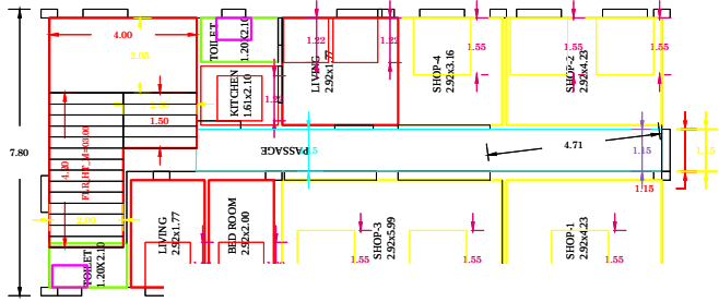
PROPOSED FIRST FLOOR PLAN BLOCK-1
