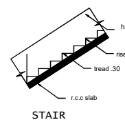
STAIR
