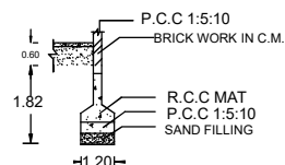
FOUNDATION DETAILS
