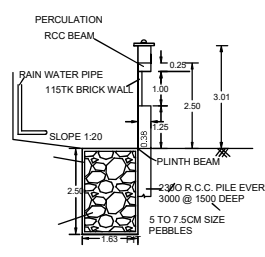
RAINWATER HARVESTING
