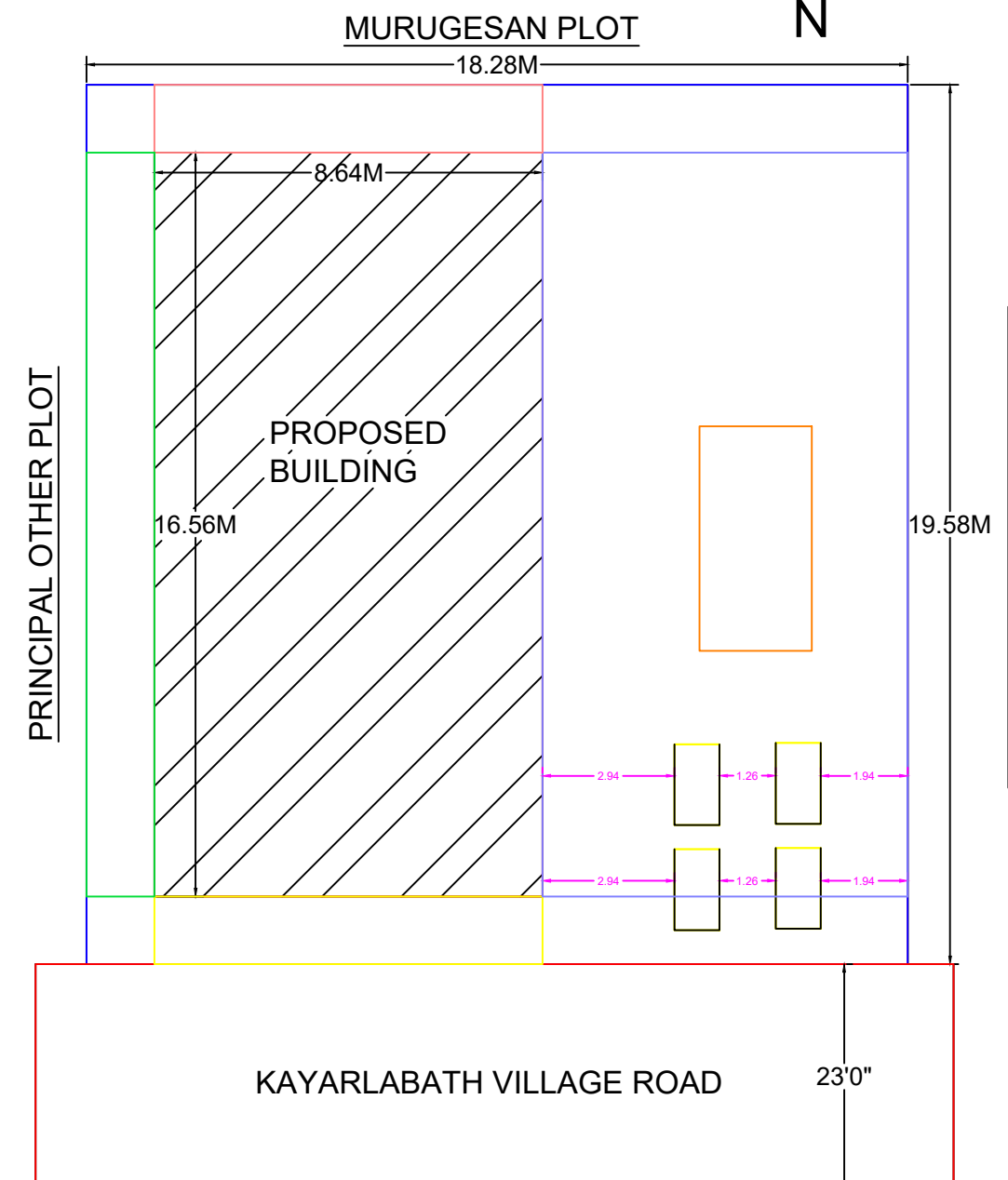
PRINCIPAL THAMBIDURAI PLOT
