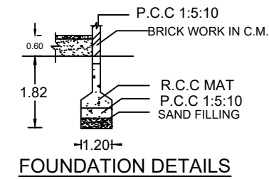
FOUNDATION DETAILS
