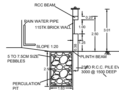
RAINWATER HARVESTING
