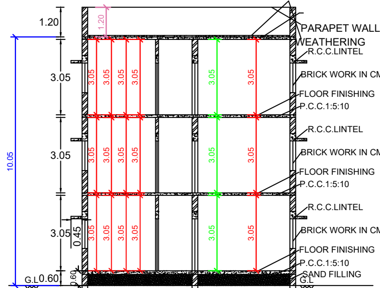
SECTION ON SS
