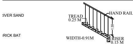
STAIRCASE DETAILS
