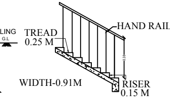
STAIRCASE DETAILS
