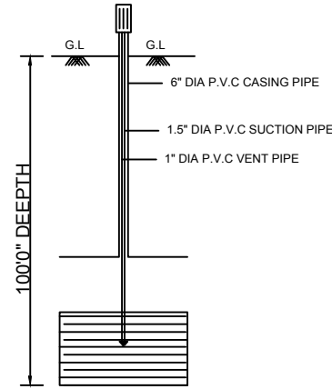
BORE WELL
