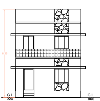
FRONT ELEVATION
