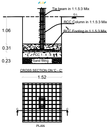
COLUMN FOUNDATION
