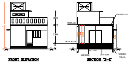
FRONT ELEVATION
