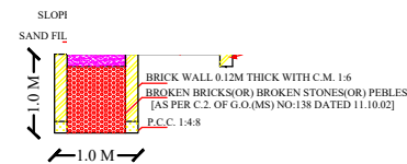
SECTION OF RAIN WATER PERCOLATION BED
