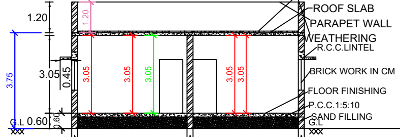
SECTION ON SS
