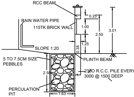
RAINWATER HARVESTING
