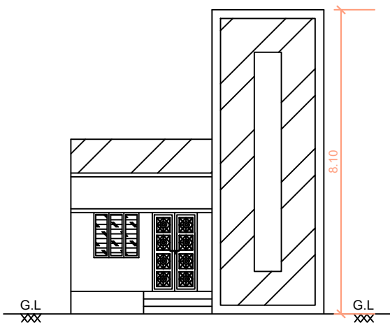
FRONT ELEVATION
