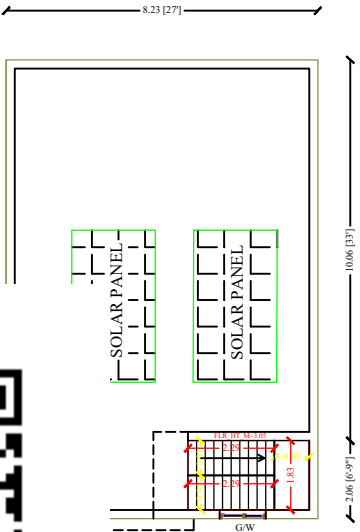
TERRACE PLAN
