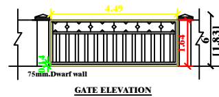
GATE ELEVATION
