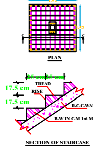
SECTION OF STAIRCASE
