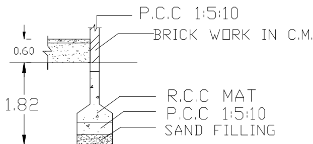
FOUNDATION DETAILS
