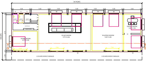
PROPOSED GROUND FLOOR PLAN
