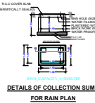
DETAILS OF COLLECTION SUM FOR RAIN PLAN
