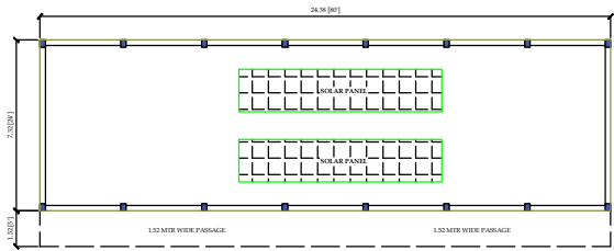
TERRACE FLOOR PLAN
