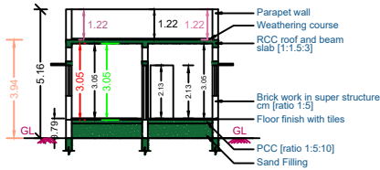
Section "AB"
