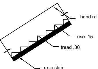
STAIR
