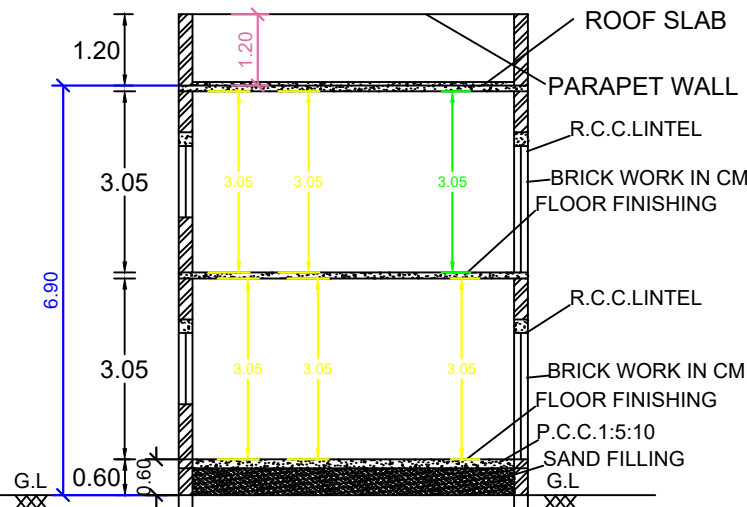
SECTION ON SS
