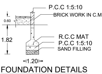
FOUNDATION DETAILS
