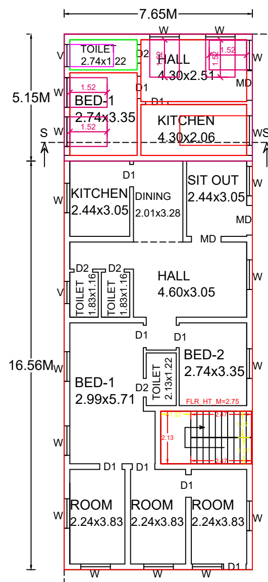
EXISTING & EXTENSION FIRST FLOOR
