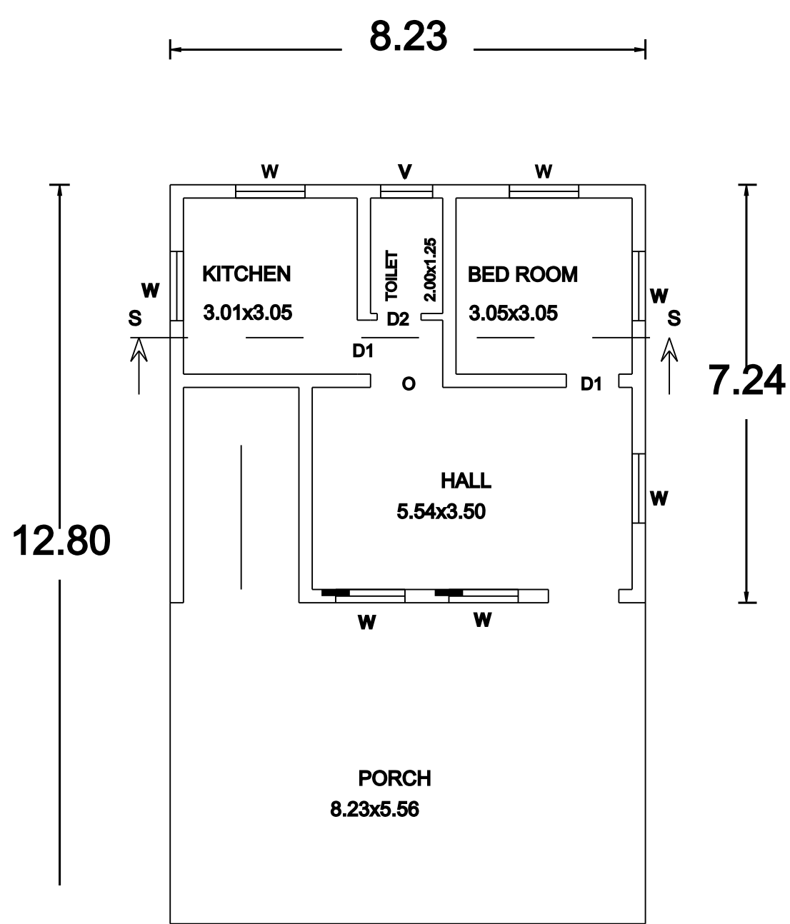
GROUND FLOOR
