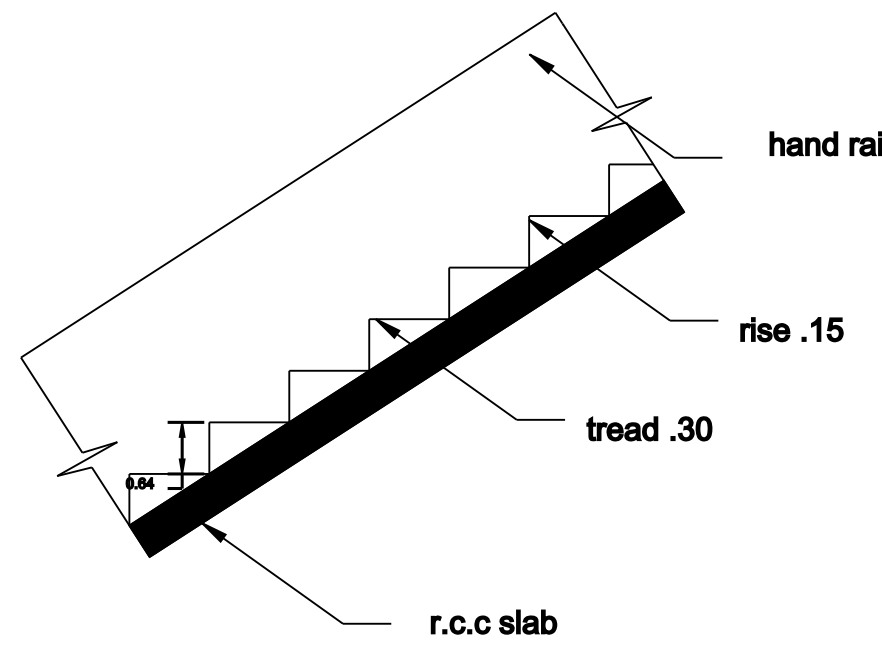
STAIR
