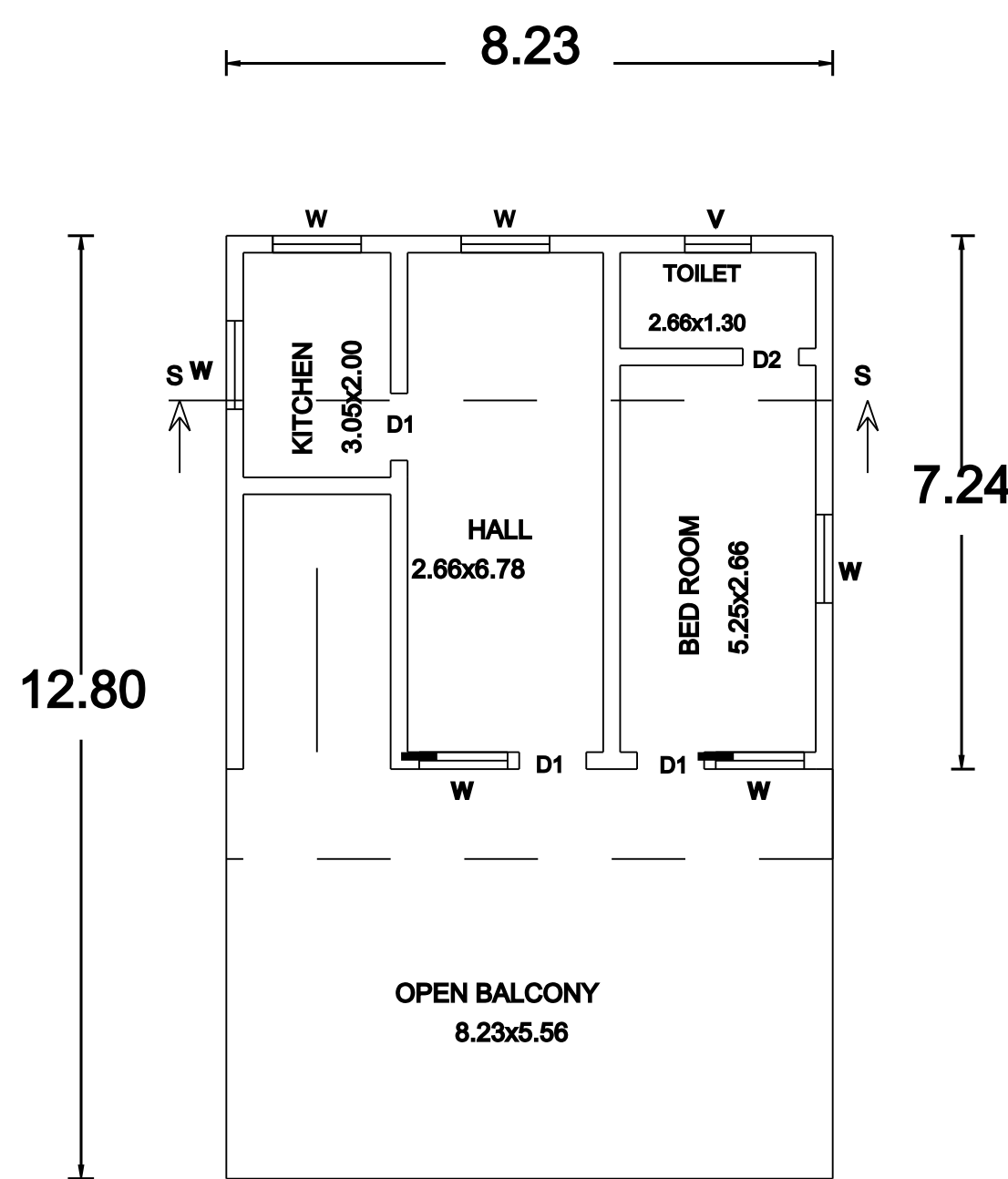
FIRST FLOOR
