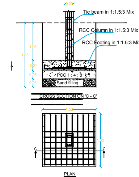
COLOUMN FOUNDATION
