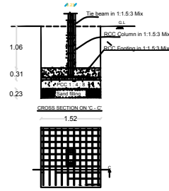
COLOUMN FOUNDATION
