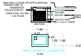
MAIN HOLE COVER (2'0" x 2'0" (0.60 x 0.60))
