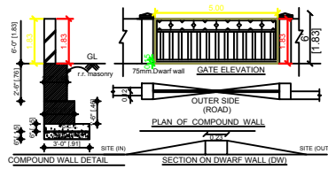
COMPOUND WALL DETAILS
