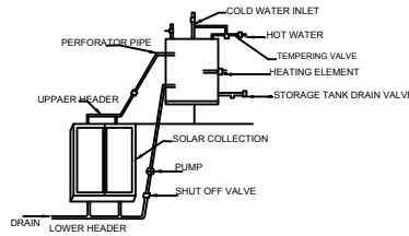
DETAILS OF SOLAR WATER HARVESTING (NTS)
