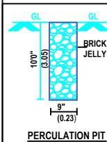
PERCOLATION PIT
