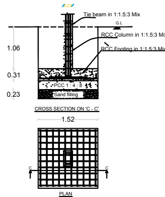
COLOUMN FOUNDATION
