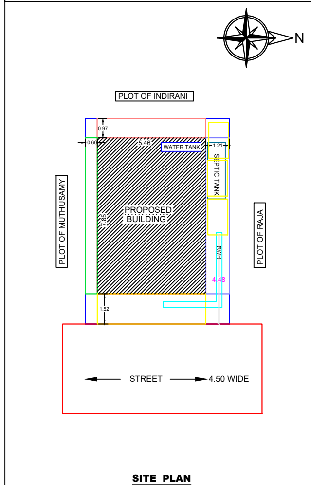
SITE PLAN
