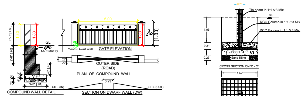
COLOUMN FOUNDATION
