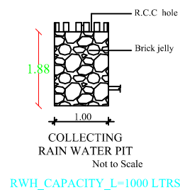
COLLECTING RAIN WATER PIT
