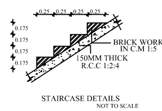
STAIRCASE DETAILS
