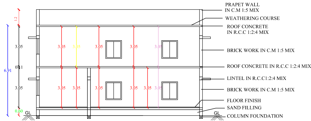
SECTION ON"XX"
